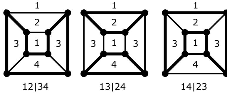
FIGURE 10. The Hamiltonian cycle of the cube
