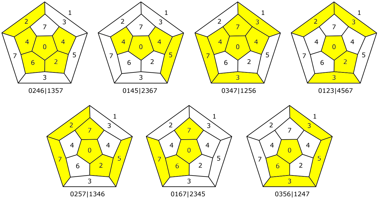
FIGURE 13. The dodecahedron with an 8-coloring producing an RHS
