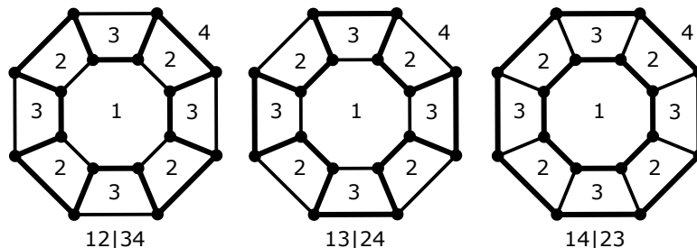
FIGURE 16. A Hamiltonian cycle on the 2k -prism
