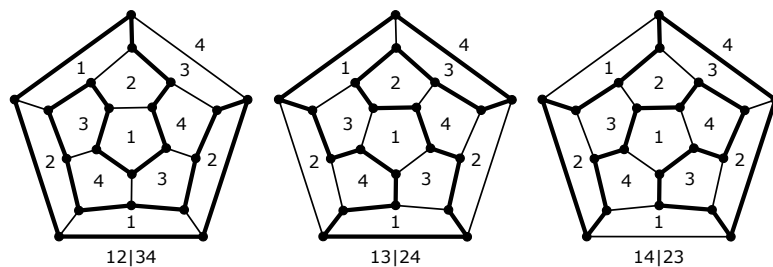
FIGURE 9. Three Hamiltonian cycles on the dodecahedron
