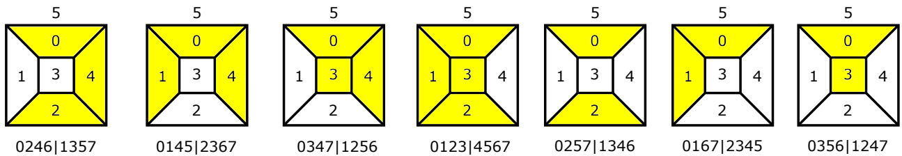
FIGURE 11. The cube with an affine coloring of rank 3 producing an RHS
