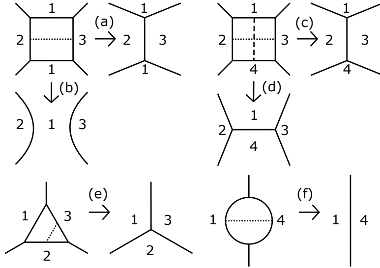
FIGURE 3. Reductions for complexes with 2 and 3 hyperelliptic involutions for r = 3 and |I(\lambda)| = 5 . By dotted and dashed lines we mark possible edges for the case r = 4 and |I(\lambda)| = 6
