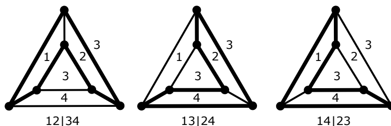
FIGURE 8. Three Hamiltonian cycles on the 3-prism
