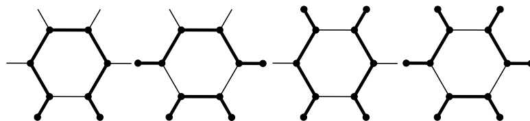
FIGURE 18. Local forms of a Hamiltonian cycle near a 6-gon
