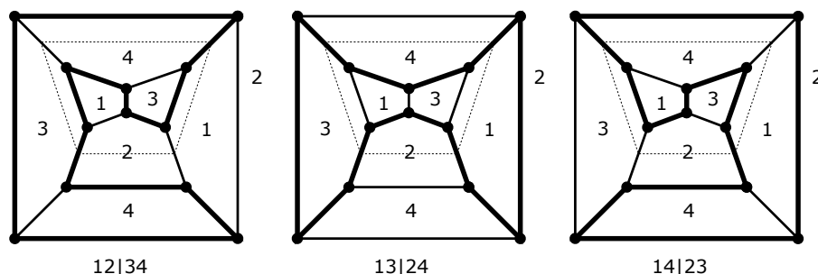
FIGURE 17. Three consistent Hamiltonian cycles on the connected sum of two 5-prisms along quadrangles
