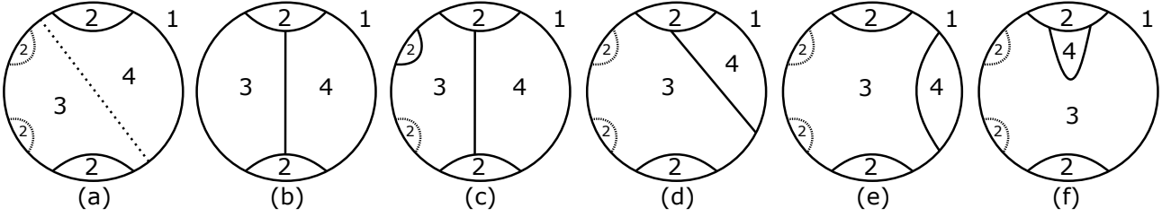
FIGURE 4. A complex \mathcal{C}(P, \lambda) when G(\mathbf{p}_1) and G(\mathbf{p}_3, \mathbf{p}_4) are intersecting disks, and G(\mathbf{p}_2) is not a disk
