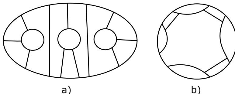
FIGURE 1. a) A subdivision of a sphere with holes; b) Cutting off the common edges
