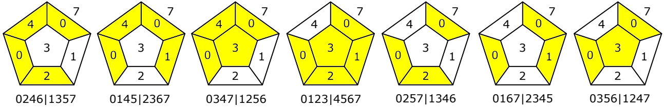
FIGURE 12. The 5-prism with an affine coloring of rank 3 producing an RHS
