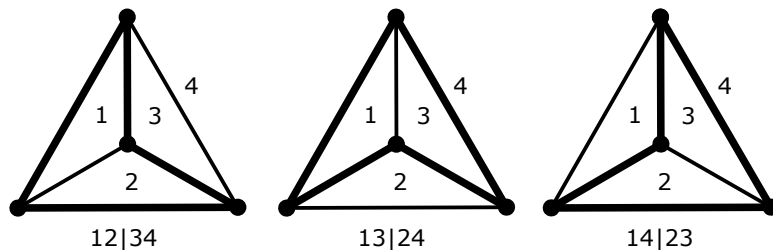
FIGURE 7. Three Hamiltonian cycles on the simplex
