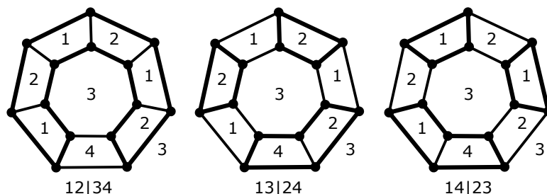
FIGURE 15. A Hamiltonian cycle on the k -prism
