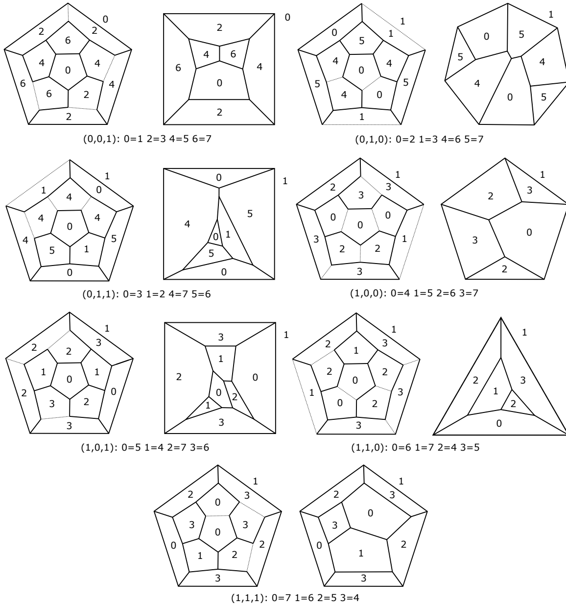
FIGURE 14. The dodecahedron with 4-colorings arising after factorisation of the 8-coloring from Fig. 13 by 1-dimensional subgroups in \mathbb{Z}_2^3 . Each subgroup is generated by a vector \mathbf{x} \in \mathbb{Z}_2^3 and gives the identification \lambda_i = \lambda_j if \lambda_i + \mathbf{x} = \lambda_j .
