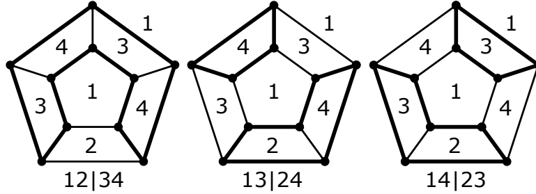
FIGURE 6. The Hamiltonian cycle on the 5-prism
