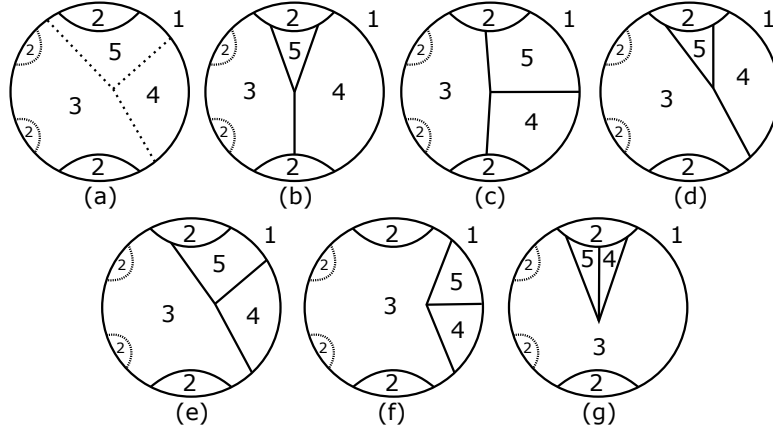
FIGURE 5. A complex \mathcal{C}(P, \lambda) when G(\mathbf{p}_1) and G(\mathbf{p}_3, \mathbf{p}_4, \mathbf{p}_4) are intersecting disks, and G(\mathbf{p}_2) is not a disk
