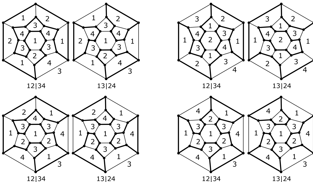
FIGURE 19. Hamiltonian cycles on the 6-barrel
