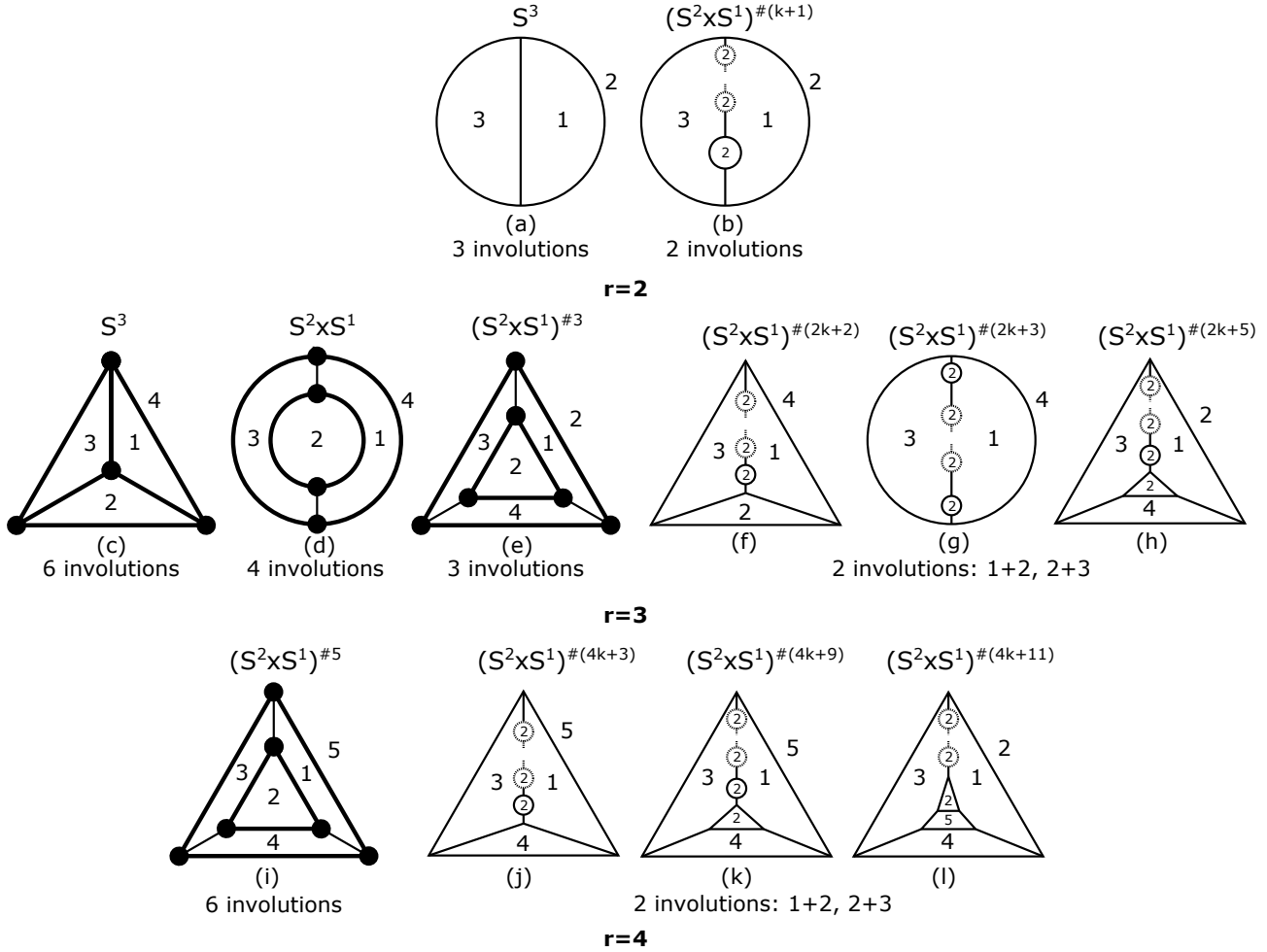
FIGURE 2. All complexes with more than one hyperelliptic involution for the case when I(\lambda) is a boolean simplex. On the top we write the homeomorphism type of N(P, \lambda) , where k \geq 0 is the number of dashed circles
